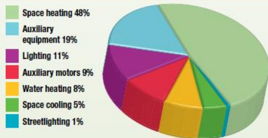
Figure 4.3 — Commercial/institutional energy use by end-use, 2008 (percent)
